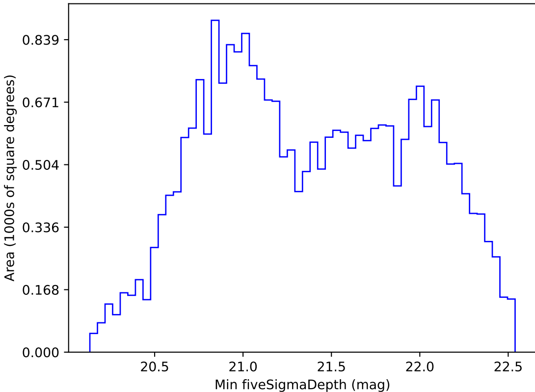
noroll_v3.4_10yrs All sky z band: Min fiveSigmaDepth
