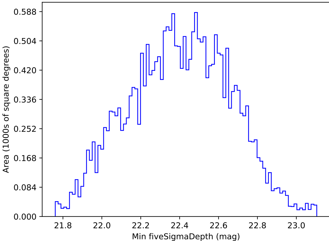
noroll_v3.4_10yrs All sky u band: Min fiveSigmaDepth
