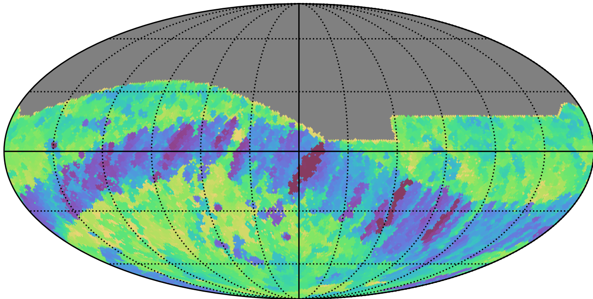
noroll_v3.4_10yrs All sky r band: Min fiveSigmaDepth
