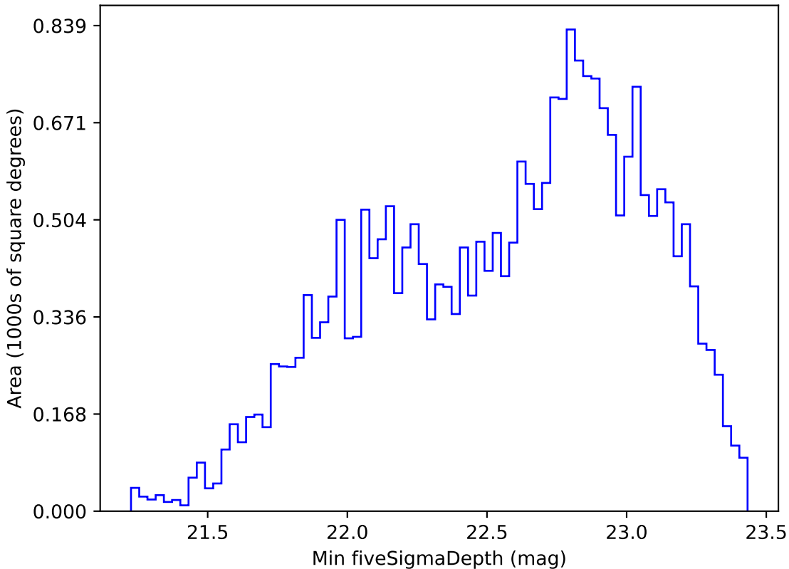
noroll_v3.4_10yrs All sky r band: Min fiveSigmaDepth
