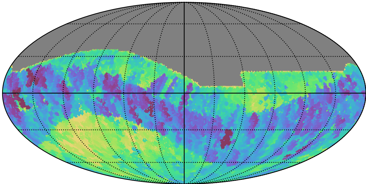
noroll_v3.4_10yrs All sky i band: Min fiveSigmaDepth
