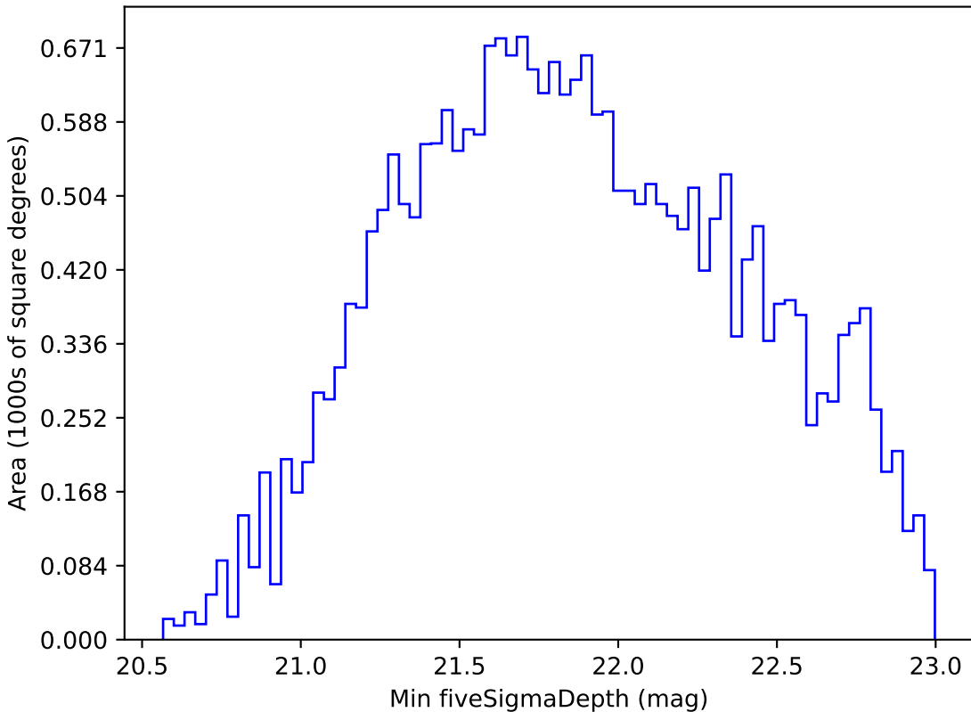
noroll_v3.4_10yrs All sky i band: Min fiveSigmaDepth
