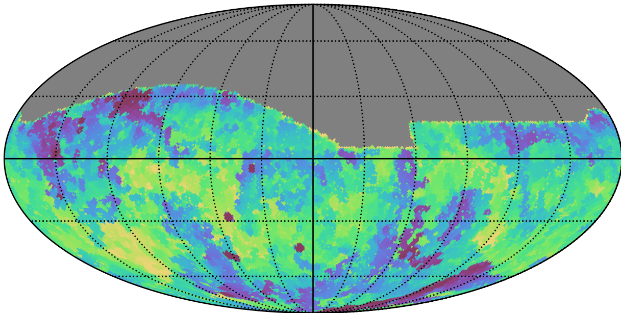
noroll_v3.4_10yrs All sky g band: Min fiveSigmaDepth
