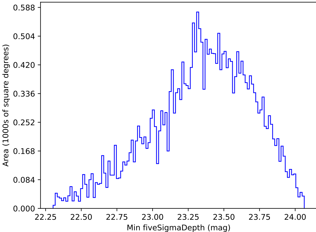
noroll_v3.4_10yrs All sky g band: Min fiveSigmaDepth
