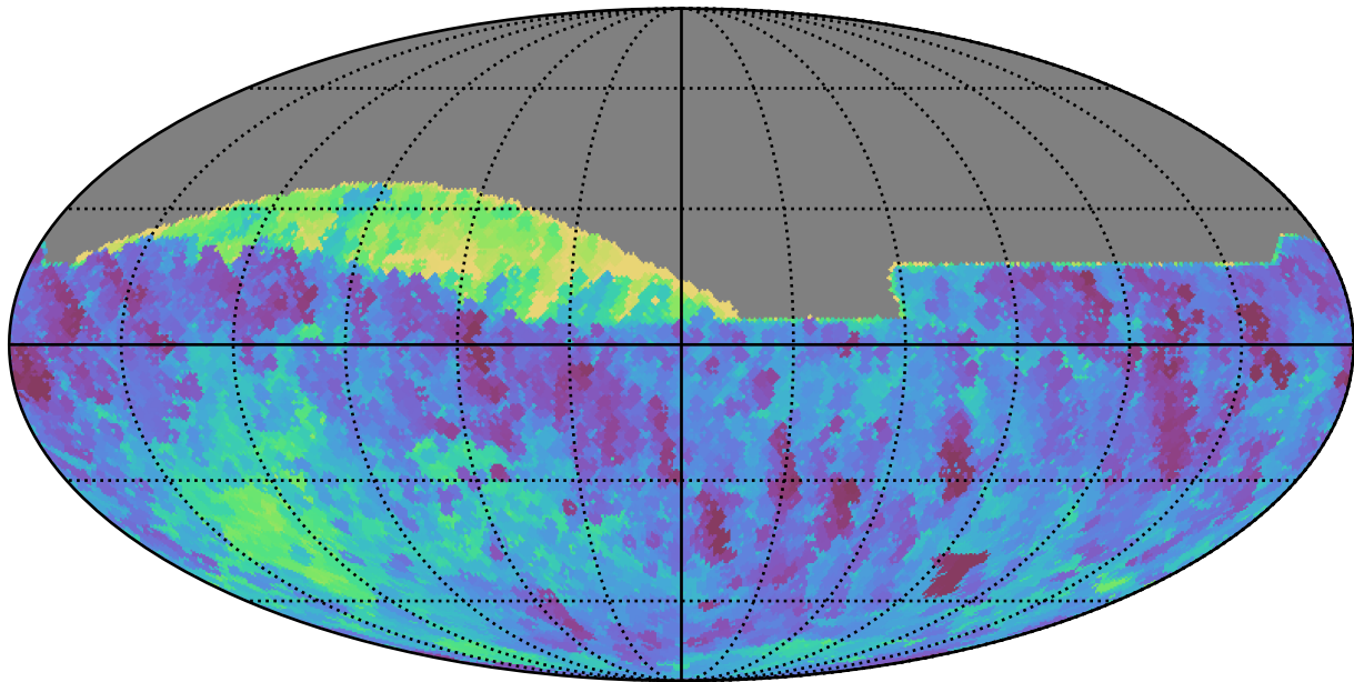
noroll_v3.4_10yrs All sky all bands: Min fiveSigmaDepth
