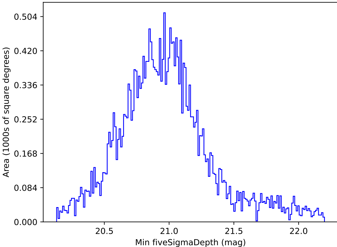
noroll_v3.4_10yrs All sky all bands: Min fiveSigmaDepth
