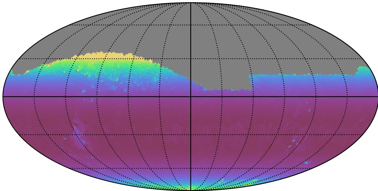
noroll_v3.4_10yrs Yr 1 z band: Min airmass
