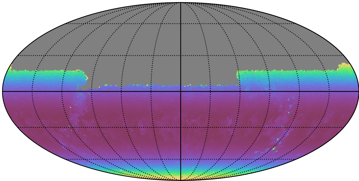
noroll_v3.4_10yrs Yr 1 y band: Min airmass
