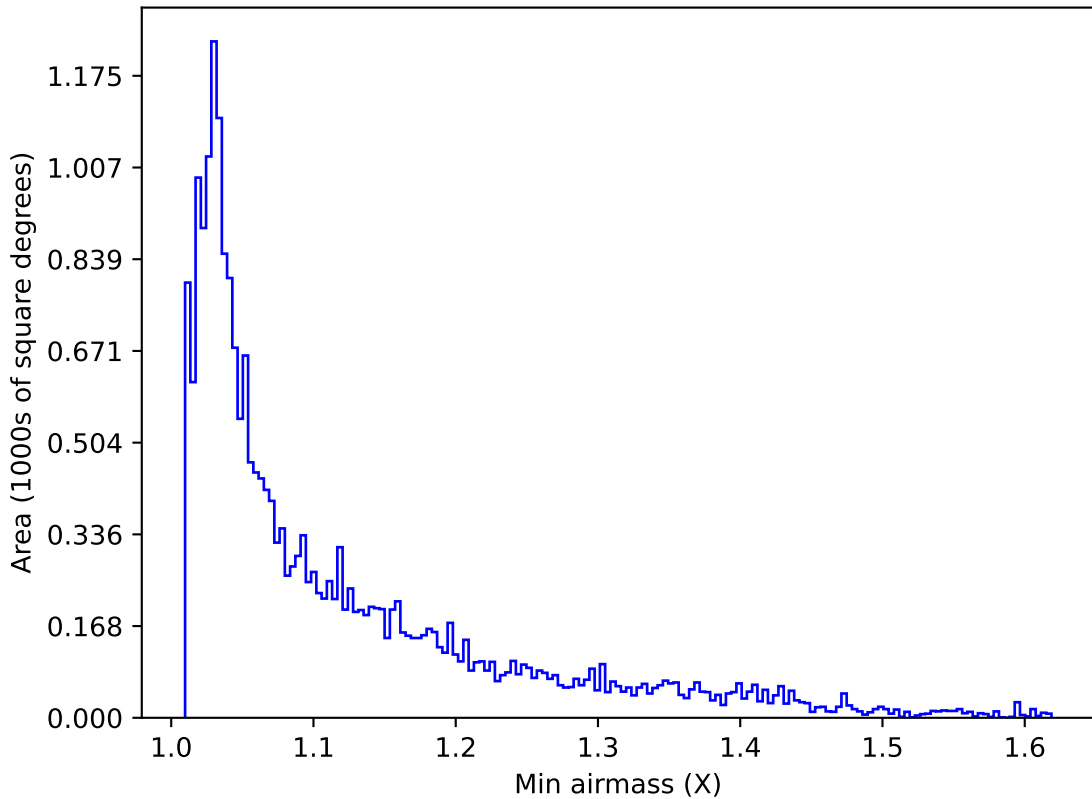
noroll_v3.4_10yrs Yr 1 y band: Min airmass
