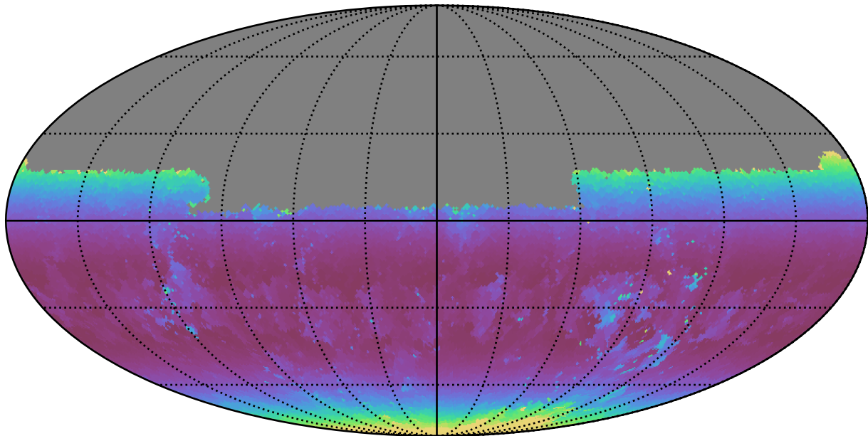
noroll_v3.4_10yrs Yr 1 u band: Min airmass
