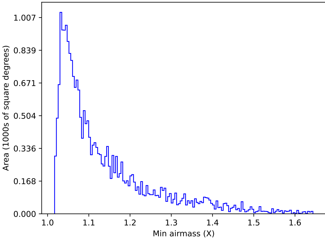
noroll_v3.4_10yrs Yr 1 u band: Min airmass
