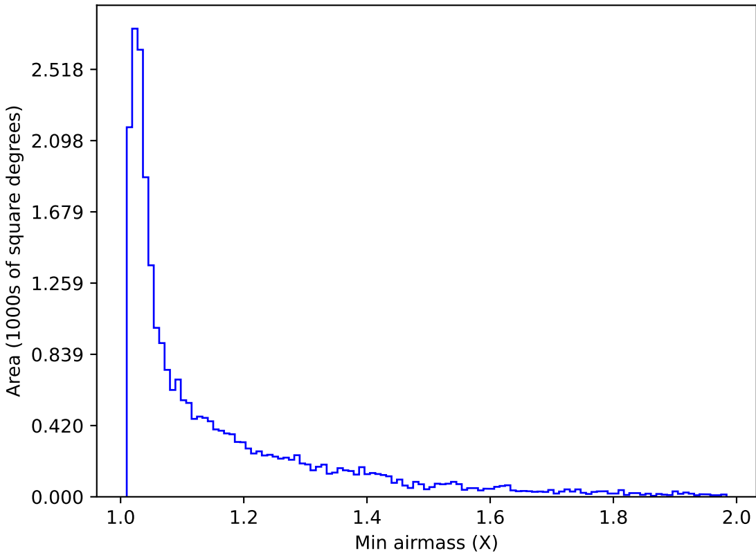
noroll_v3.4_10yrs Yr 1 r band: Min airmass
