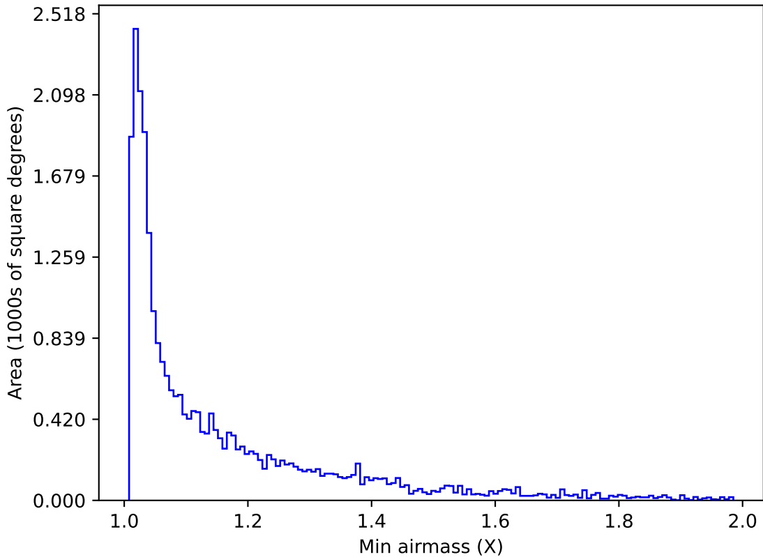
noroll_v3.4_10yrs Yr 1 i band: Min airmass
