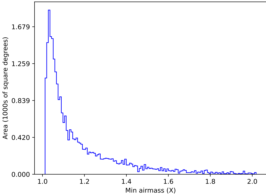
noroll_v3.4_10yrs Yr 1 g band: Min airmass
