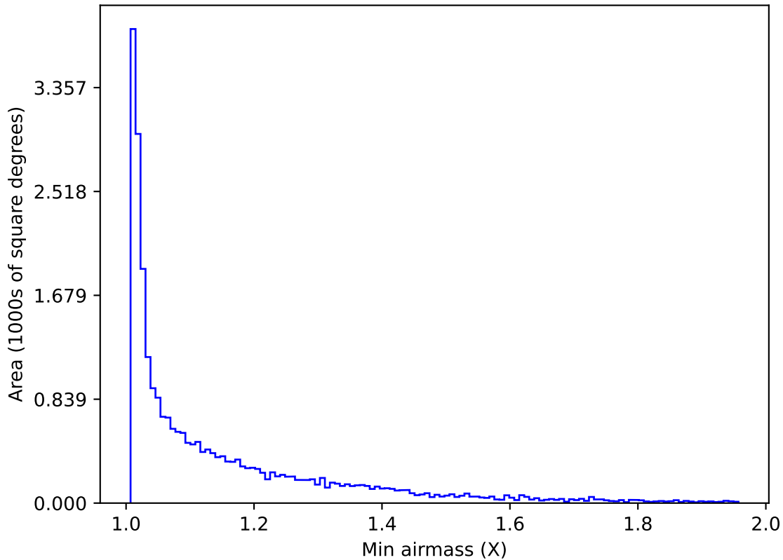
noroll_v3.4_10yrs Yr 1 all bands: Min airmass
