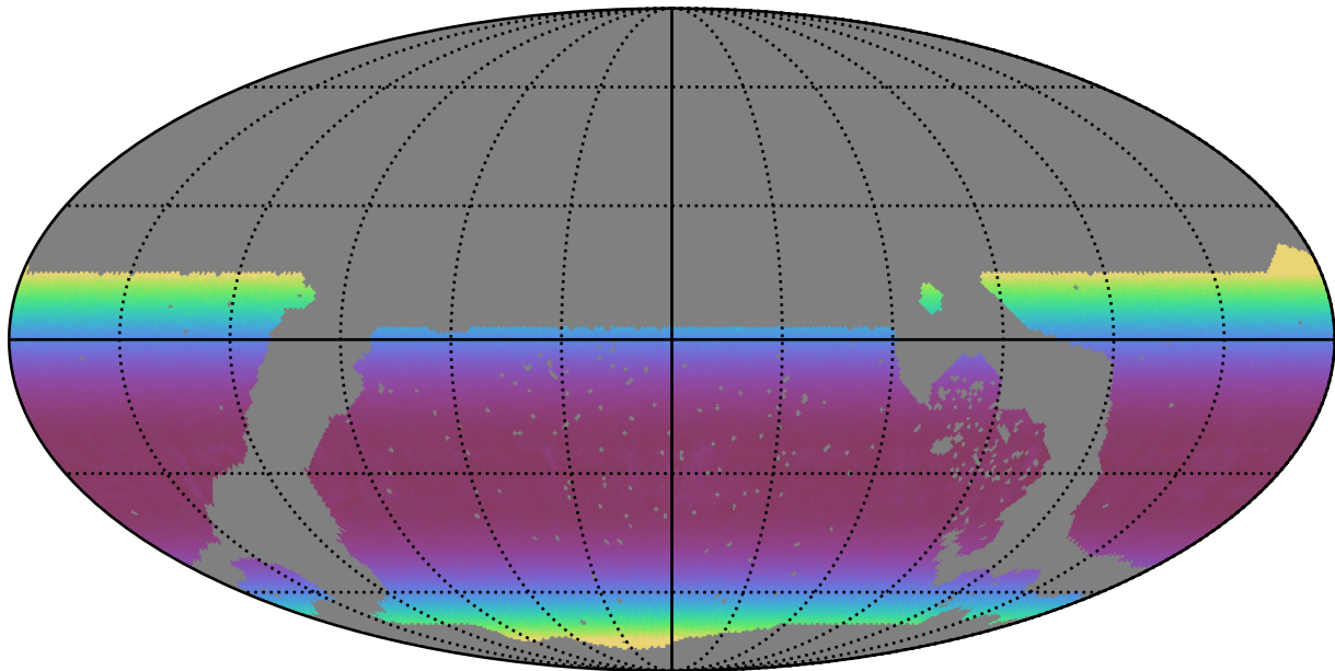
noroll_v3.4_10yrs WFD z band: Min airmass
