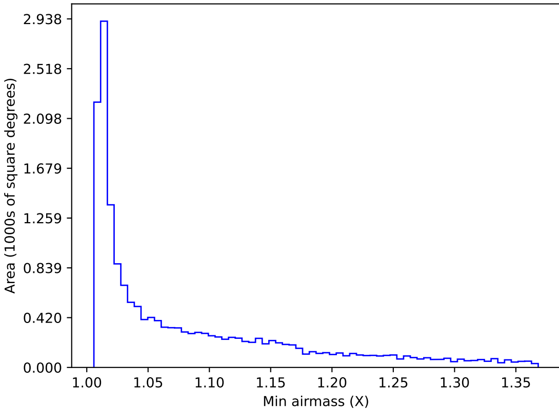
noroll_v3.4_10yrs WFD z band: Min airmass
