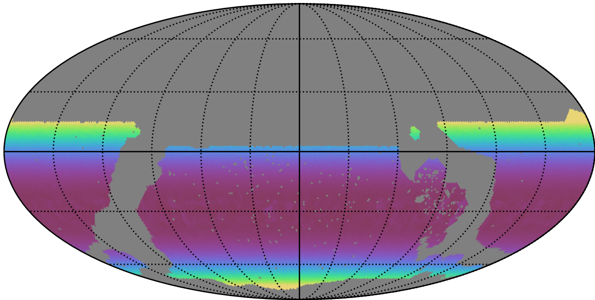
noroll_v3.4_10yrs WFD y band: Min airmass
