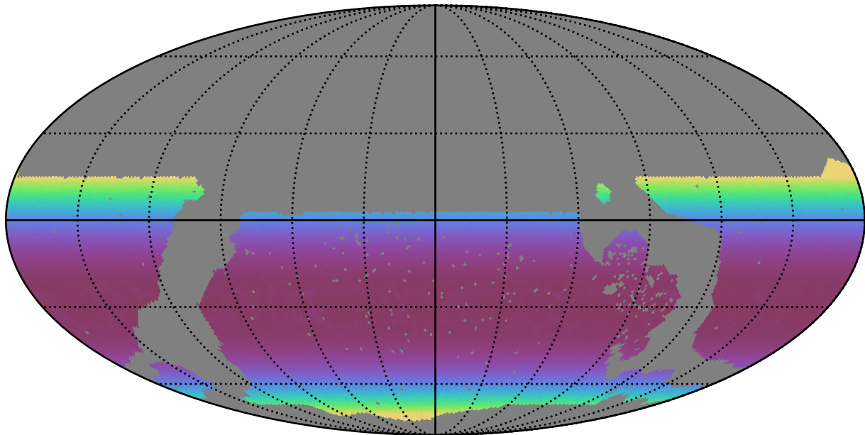
noroll_v3.4_10yrs WFD r band: Min airmass
