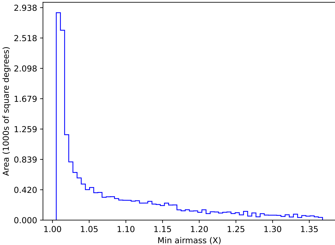
noroll_v3.4_10yrs WFD r band: Min airmass
