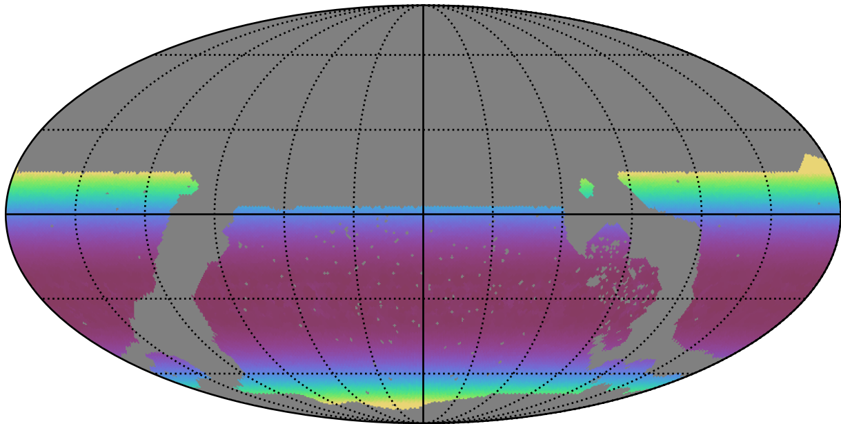
noroll_v3.4_10yrs WFD i band: Min airmass
