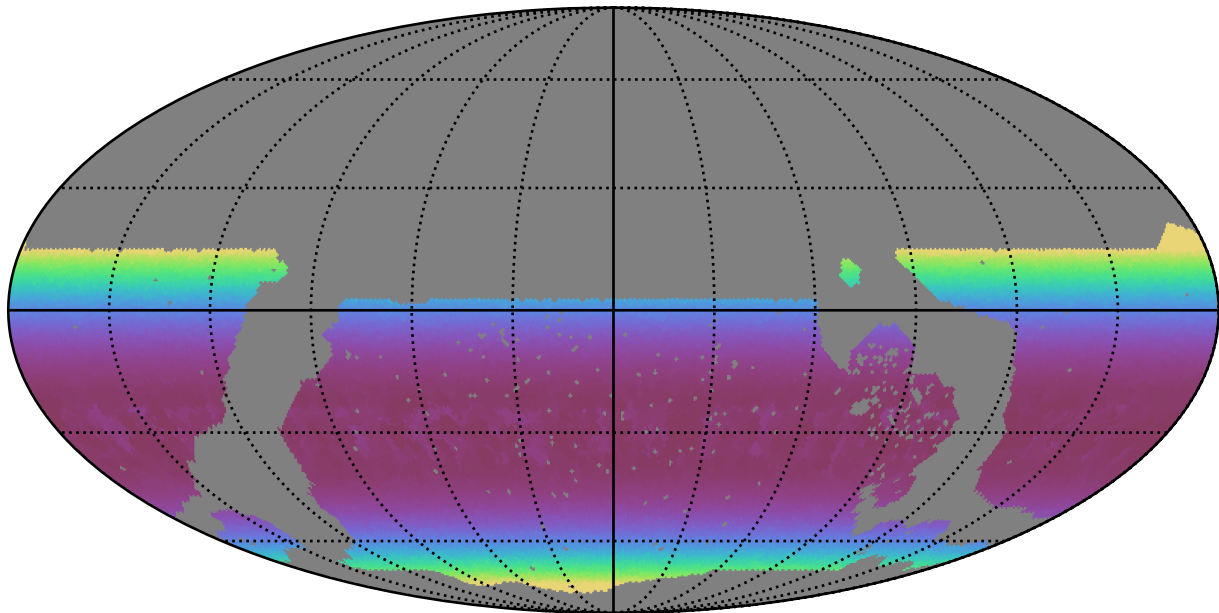
noroll_v3.4_10yrs WFD g band: Min airmass
