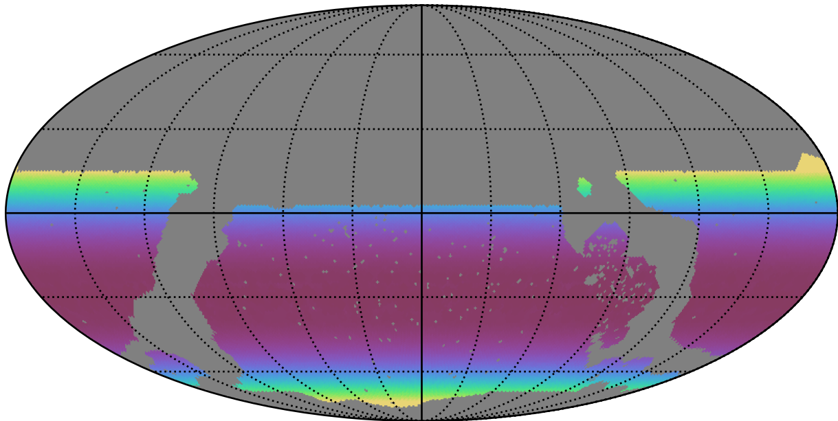
noroll_v3.4_10yrs WFD all bands: Min airmass
