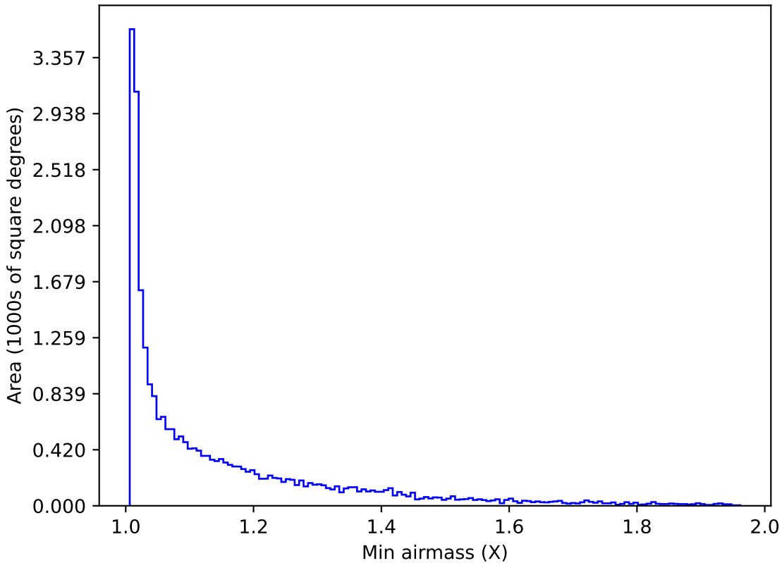
noroll_v3.4_10yrs All sky z band: Min airmass
