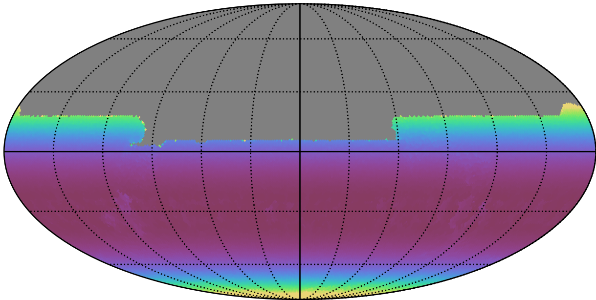
noroll_v3.4_10yrs All sky y band: Min airmass
