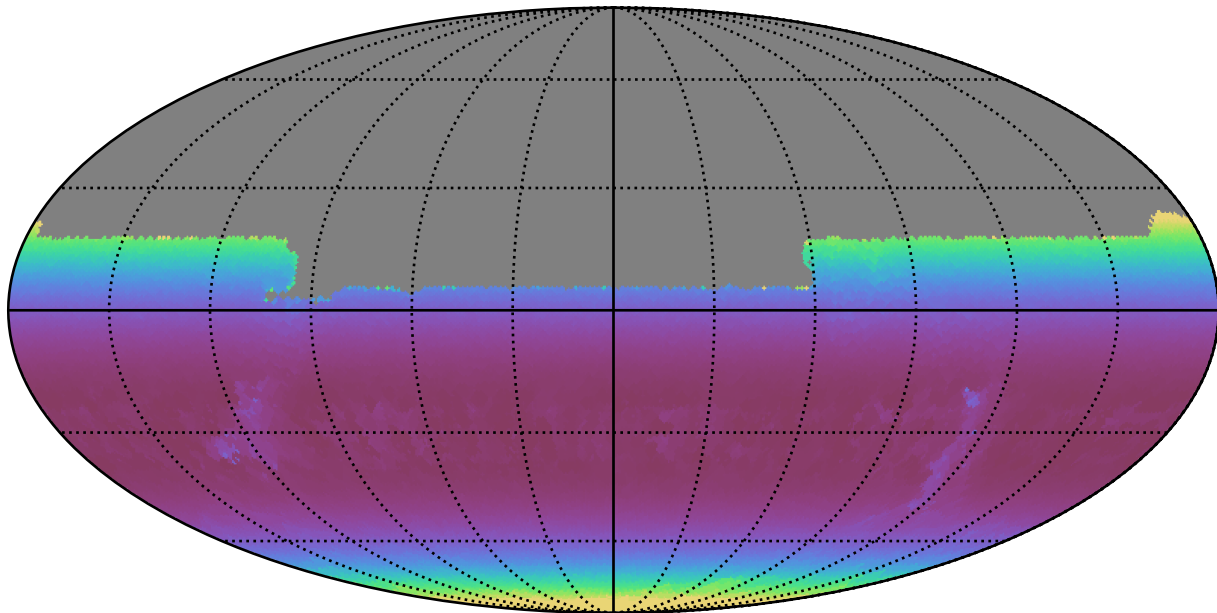
noroll_v3.4_10yrs All sky u band: Min airmass
