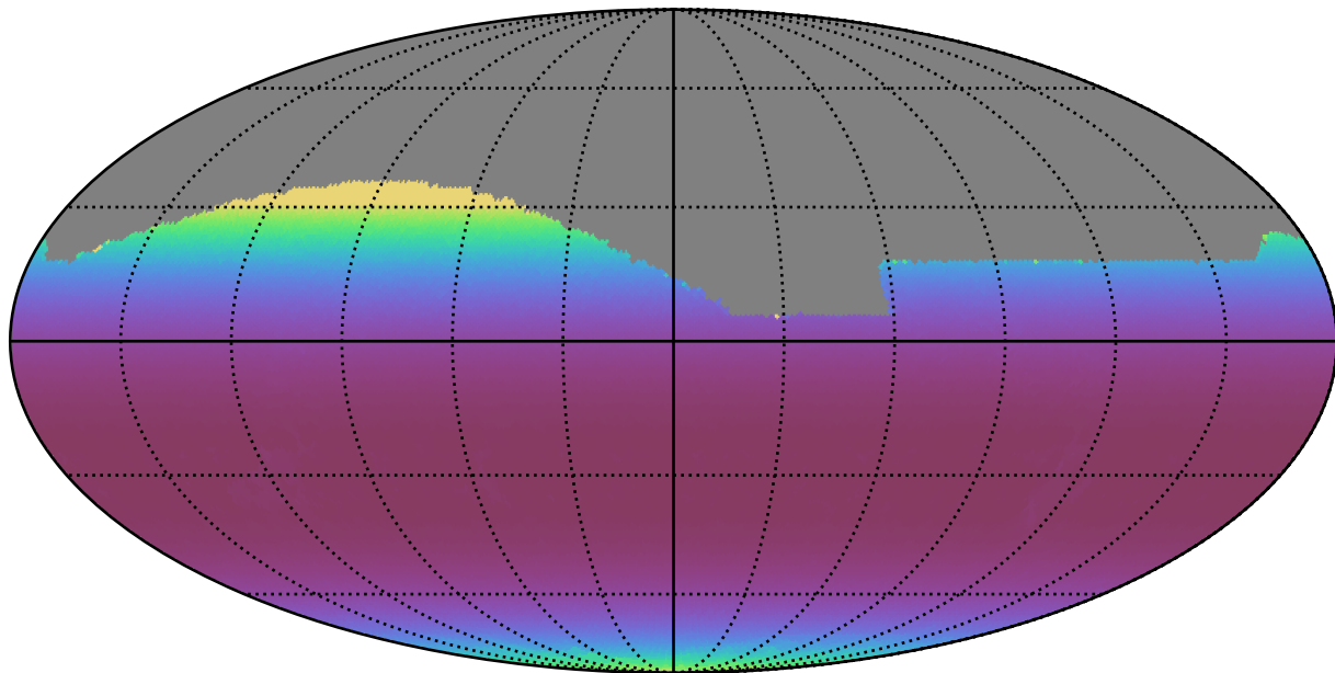
noroll_v3.4_10yrs All sky r band: Min airmass
