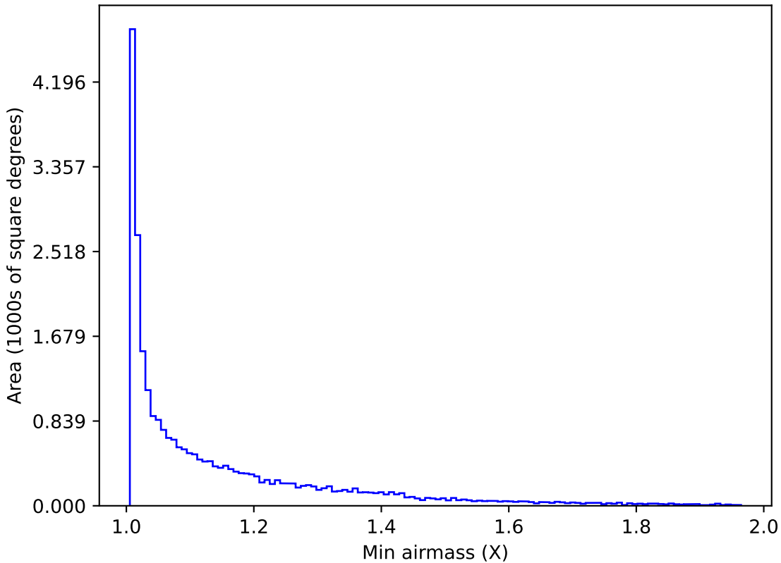
noroll_v3.4_10yrs All sky r band: Min airmass
