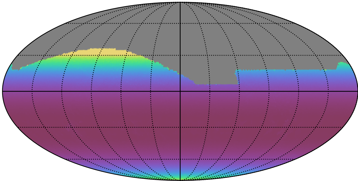
noroll_v3.4_10yrs All sky i band: Min airmass
