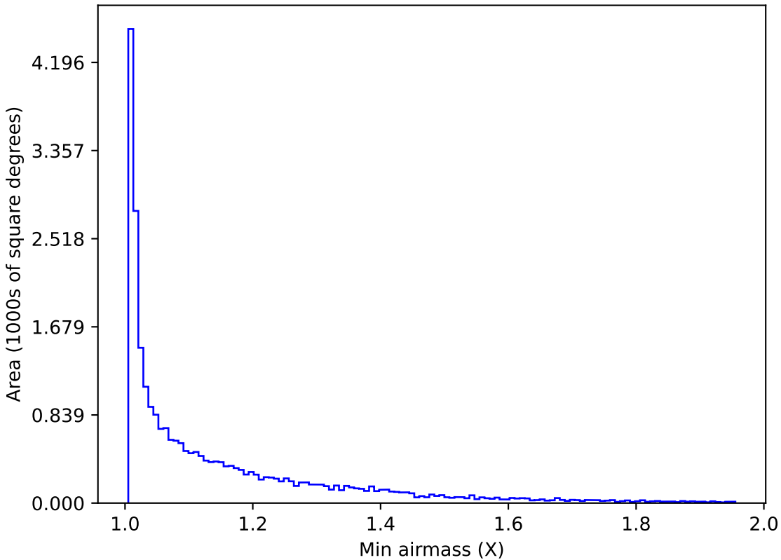
noroll_v3.4_10yrs All sky i band: Min airmass
