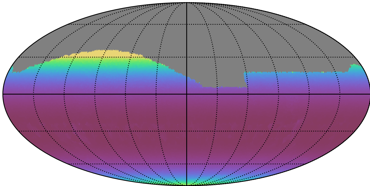
noroll_v3.4_10yrs All sky g band: Min airmass
