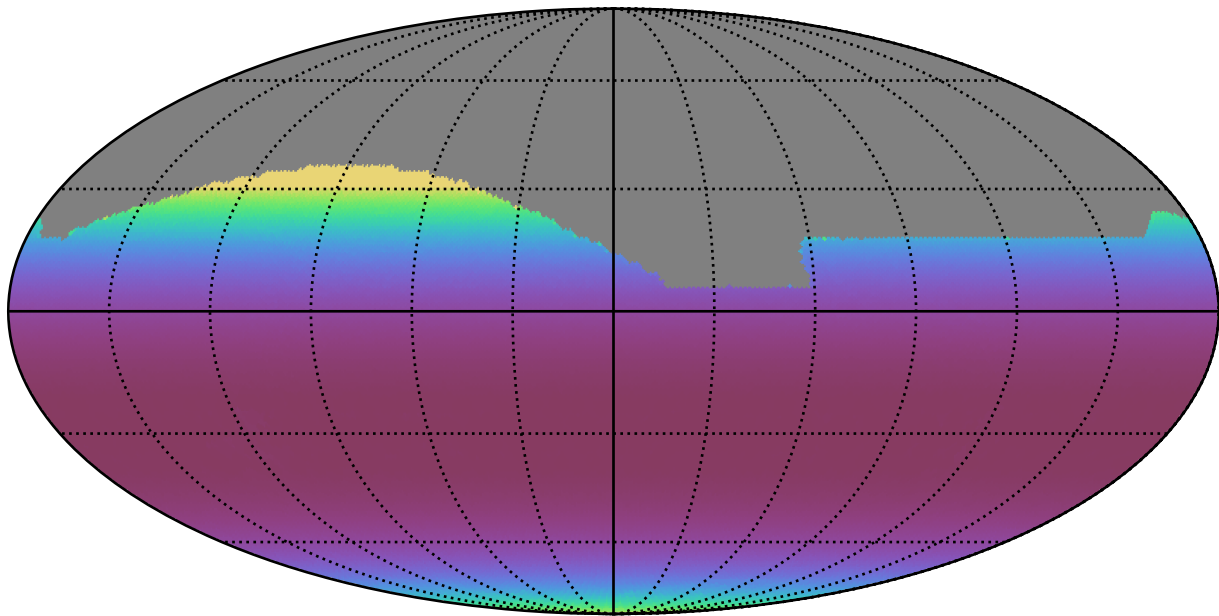
noroll_v3.4_10yrs All sky all bands: Min airmass
