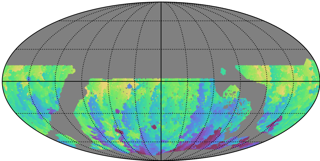
noroll_v3.4_10yrs WFD u band: Min HA
