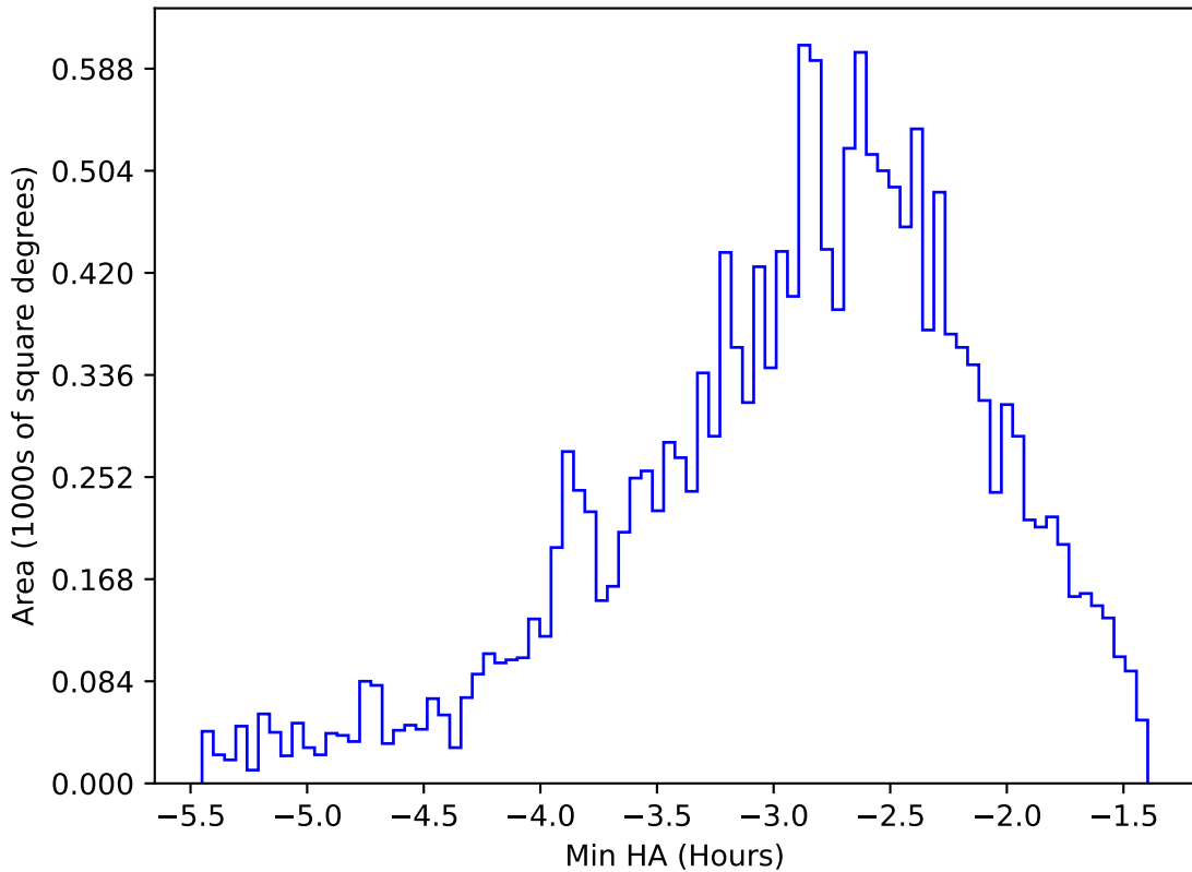
noroll_v3.4_10yrs WFD u band: Min HA
