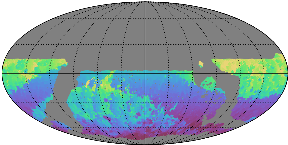
noroll_v3.4_10yrs WFD r band: Min HA
