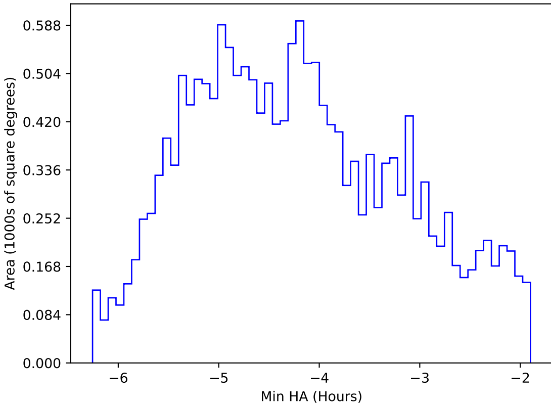
noroll_v3.4_10yrs WFD r band: Min HA
