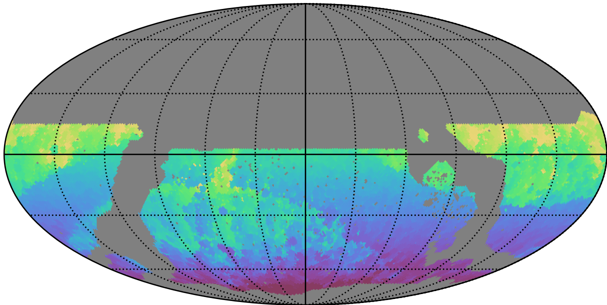
noroll_v3.4_10yrs WFD all bands: Min HA
