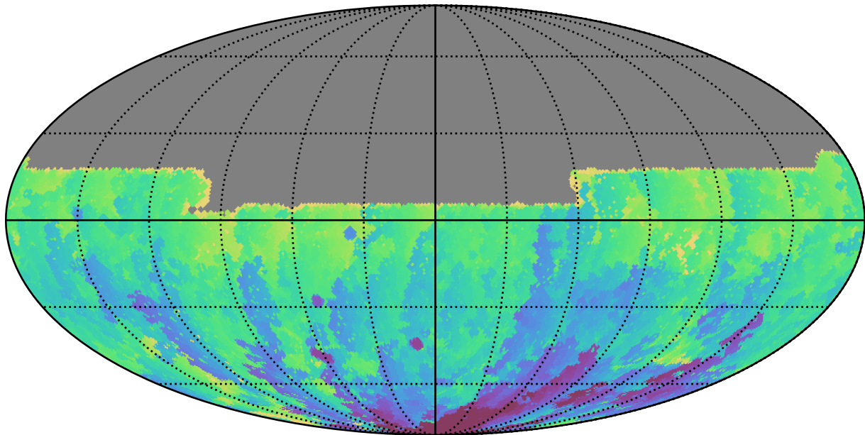
noroll_v3.4_10yrs All sky u band: Min HA
