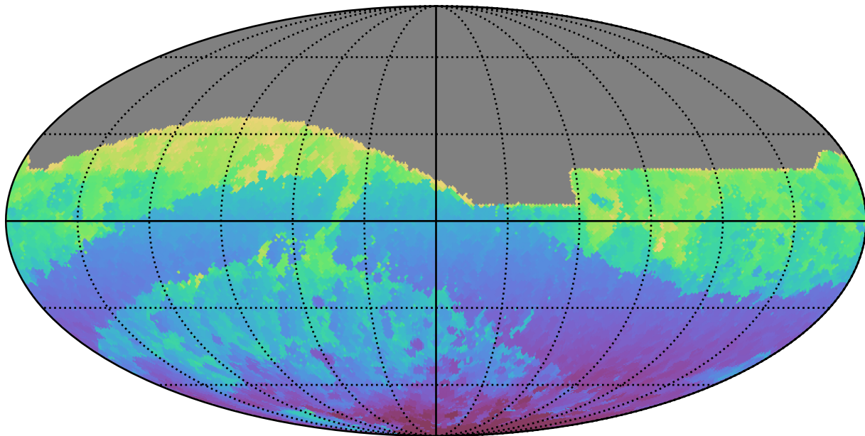
noroll_v3.4_10yrs All sky r band: Min HA
