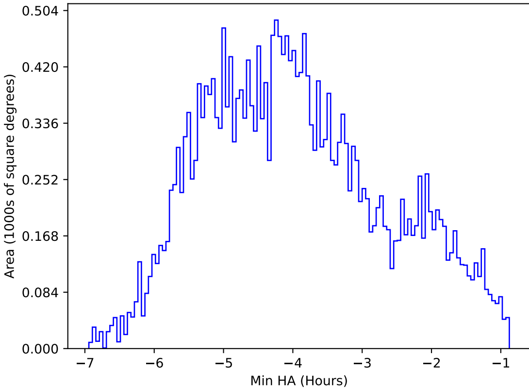
noroll_v3.4_10yrs All sky r band: Min HA
