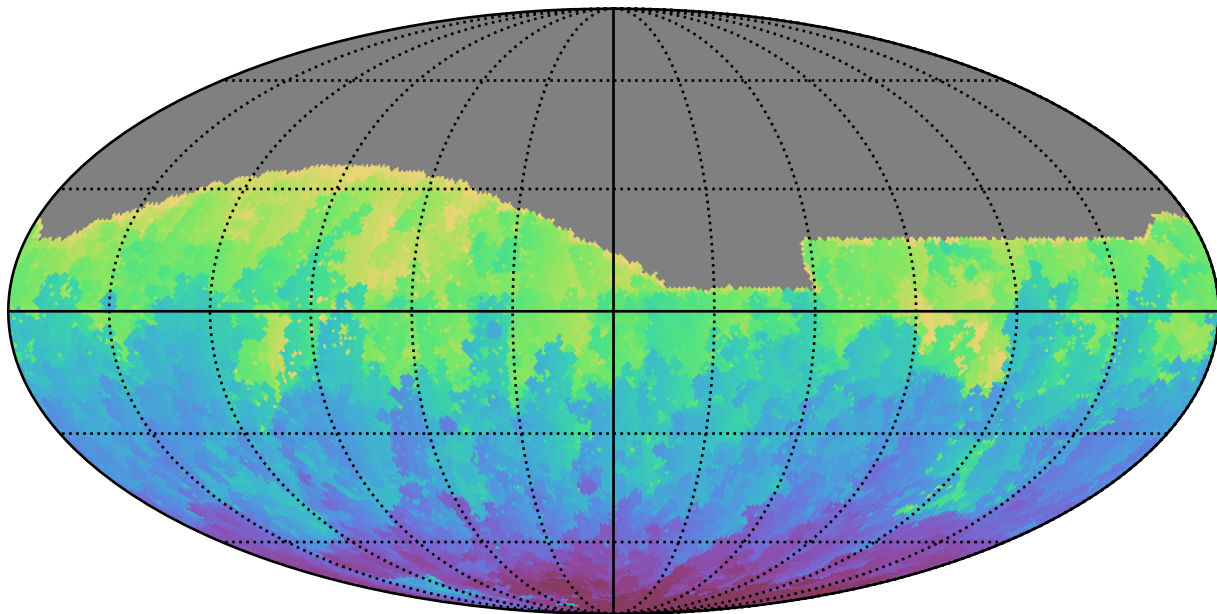
noroll_v3.4_10yrs All sky g band: Min HA
