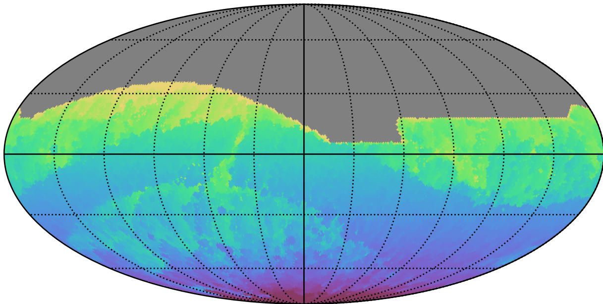
noroll_v3.4_10yrs All sky all bands: Min HA
