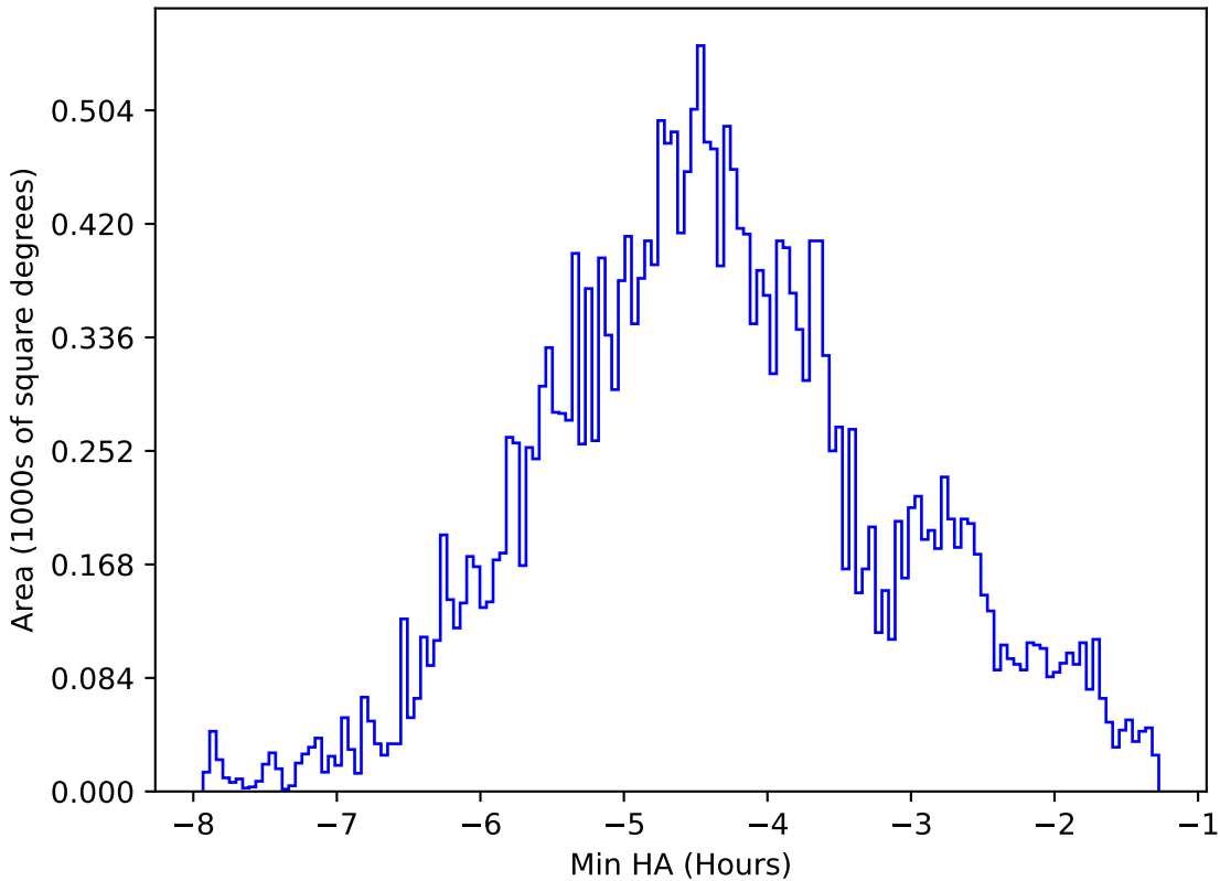
noroll_v3.4_10yrs All sky all bands: Min HA
