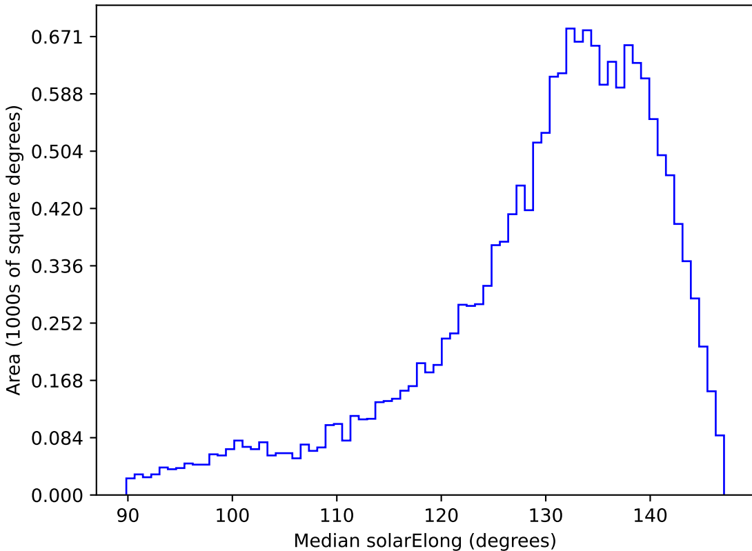
noroll_v3.4_10yrs WFD y band: Median solarElong
