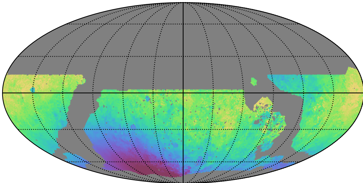
noroll_v3.4_10yrs WFD u band: Median solarElong
