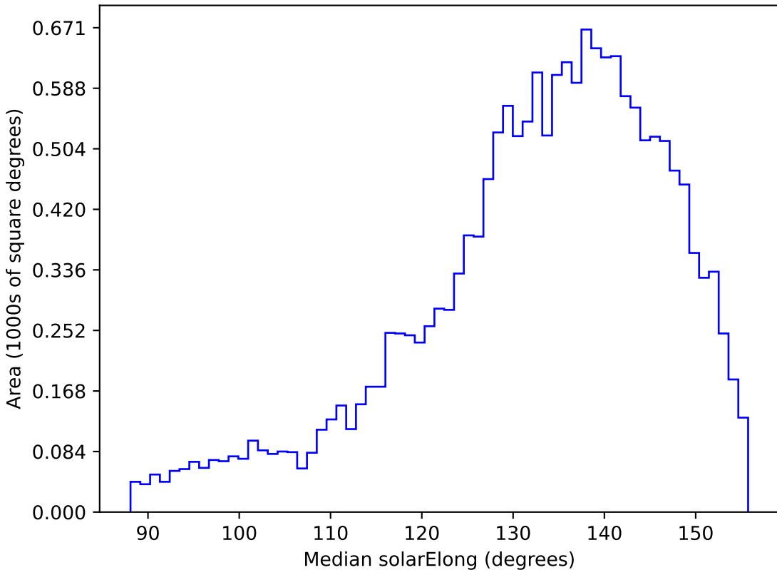
noroll_v3.4_10yrs WFD u band: Median solarElong
